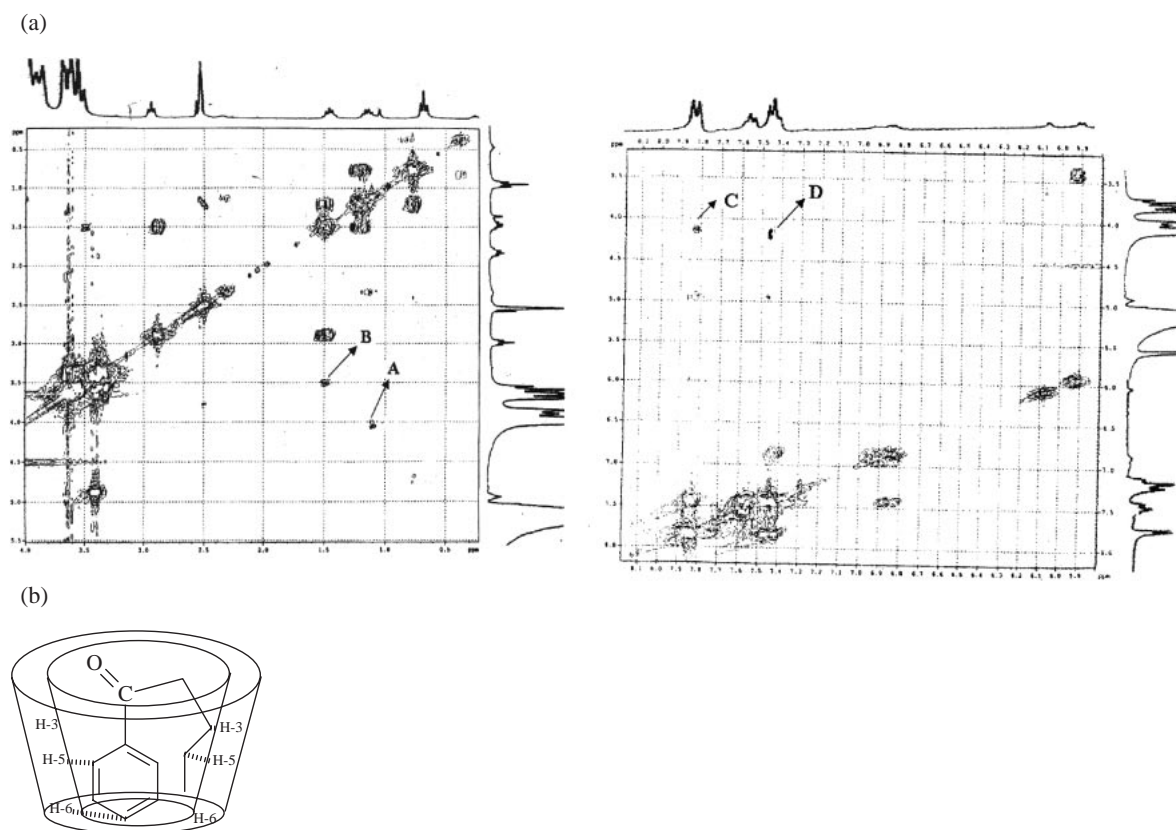
Fig. 4. (a) ^1\text{H} - ^1\text{H} NOESY spectra of \gamma -CD/valerophenone ( 1 ) in \text{D}_2\text{O} at 25^\circ\text{C} . (b) Possible orientation of 1 in \gamma -CD cavity.
