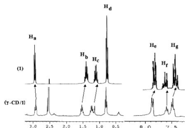
Fig. 3. ^1\text{H} NMR spectra of 1 and its \gamma -CD complex in \text{D}_2\text{O} at 25^\circ\text{C} .
