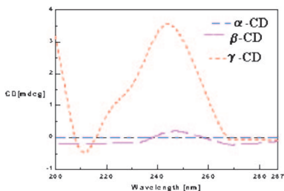
Fig. 2. ICD spectra of valerophenone ( 0.5 \times 10^{-4} M) in presence of \alpha -, \beta -, and \gamma -CDs ( 4 \times 10^{-3} M).
