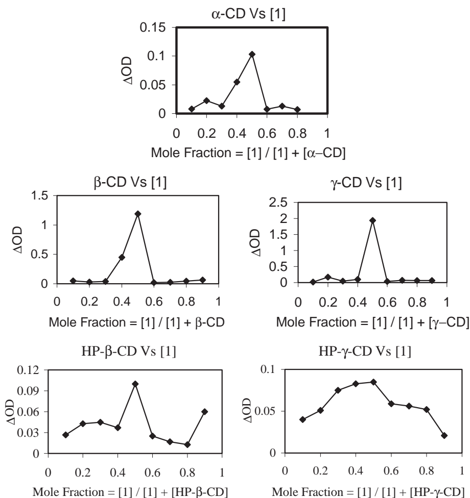
Fig. 1. Job's plots for valerophenone (1) in presence of various cyclodextrins.
